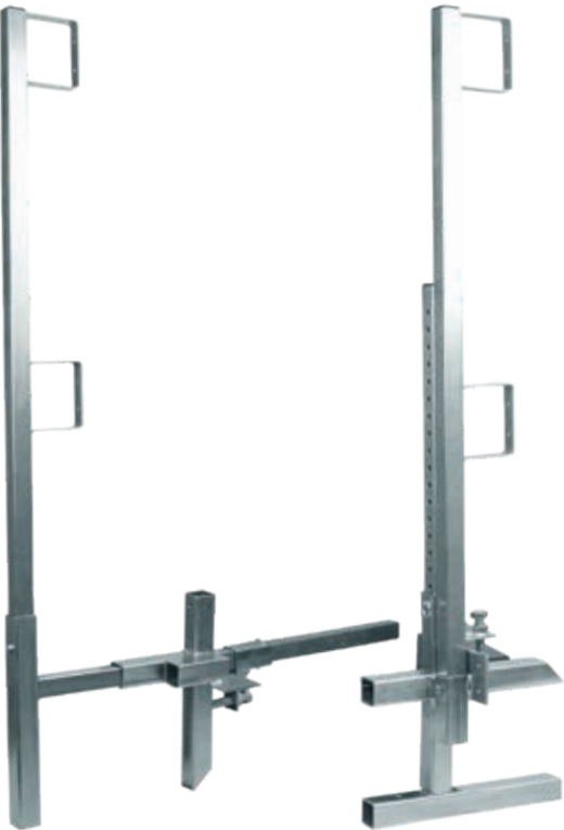
Guardrail assembly shown in parapet wall application.
