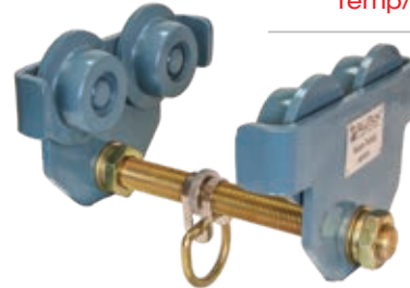
7711 Heavy Duty Beam Trolley
