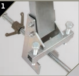
1 Clamp and wing nut installation.
